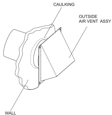
Caulk And Install Duct Termination Figure 18
