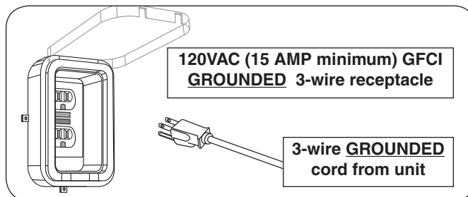
Fig. 18-4 Electrical setup detail
