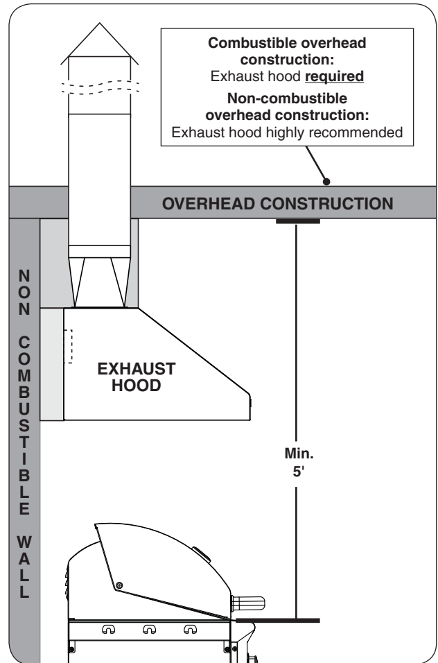
Fig. 8-1 Overhead requirements
