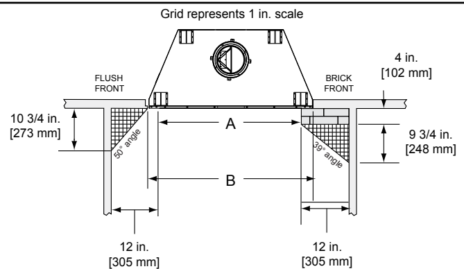
Figure 8.4 Mantel Specifications
