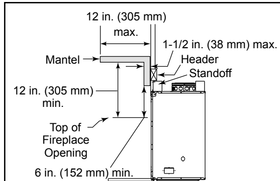
Figure 8.4 Mantel Specifications
