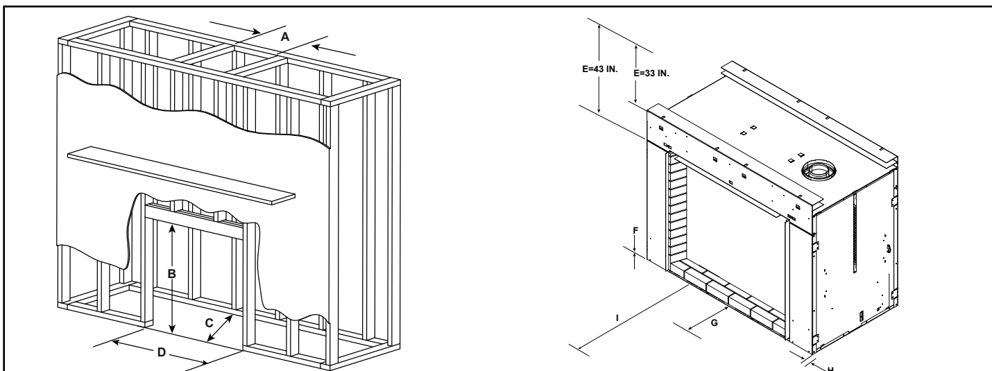
MINIMUM FRAMING DIMENSIONS*
