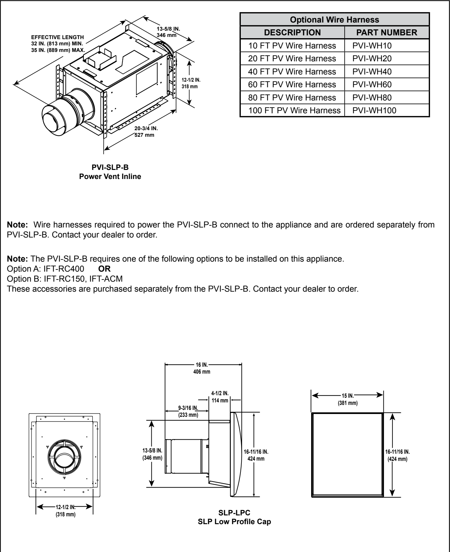
Figure 12.5 Vent Components
