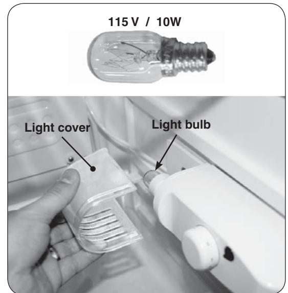
Fig. 13-1 Replace light bulb
