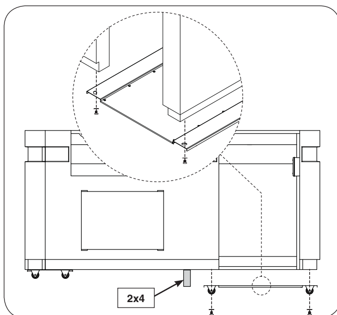
Fig. 2-4 Install right wheel assembly
