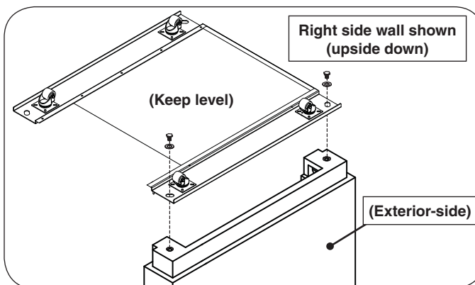
Fig. 1-2 Install right wheel assembly to bottom of right side wall
