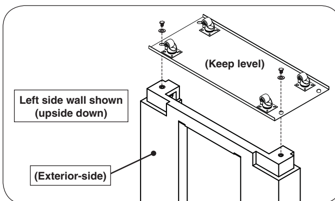
Fig. 1-1 Install left wheel assembly to bottom of left side wall
