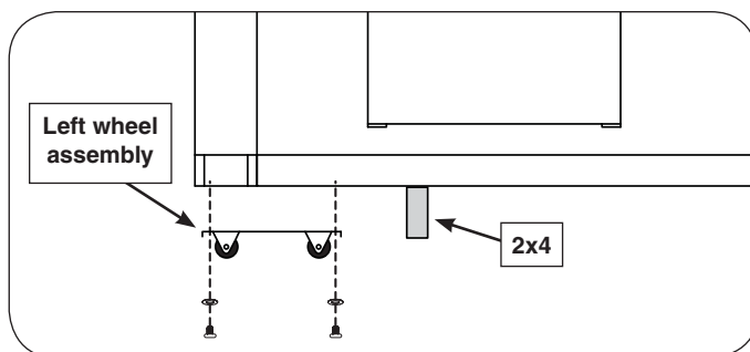
Fig. 2-3 Install left wheel assembly
