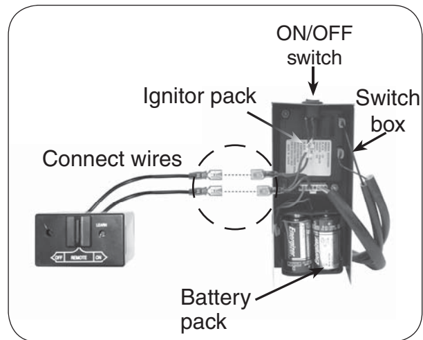
Fig. 9-1 Switch box detail
