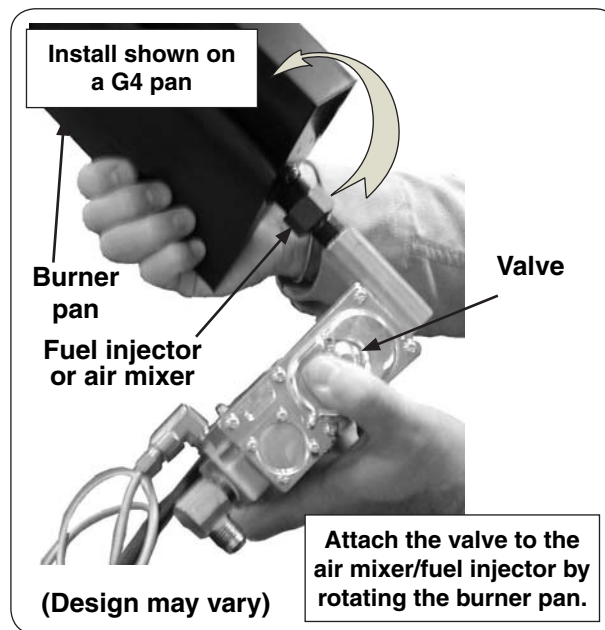
Fig. 5-1 Install valve
