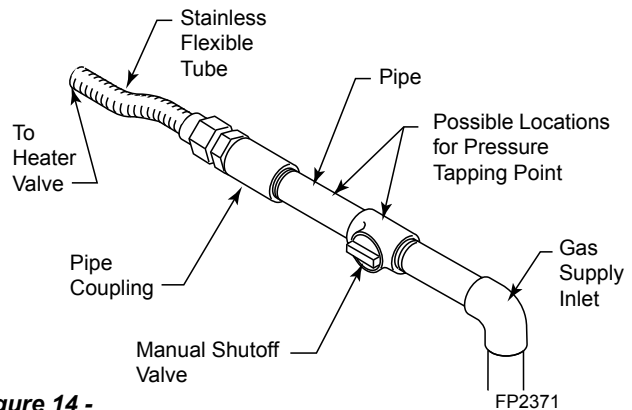
Figure 14 - Gas Connection
