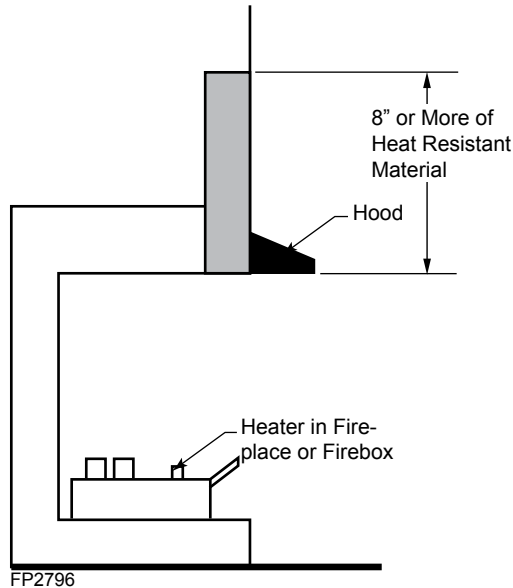
Figure 5 - Measure Heat Resistant Material for Mantel
