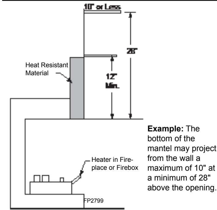
Figure 8 - DEB24/30 Minimum Mantel Clearance with No Hood
