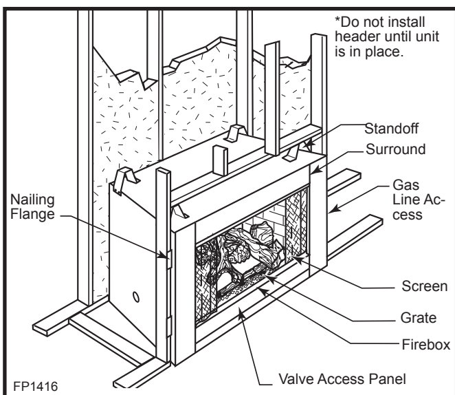
Fig. 8 Parts identification.
