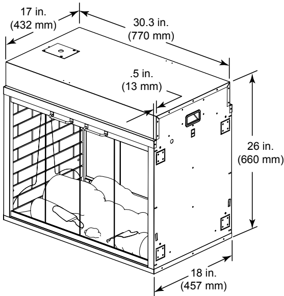
SFE-ST Appliance Dimensions
