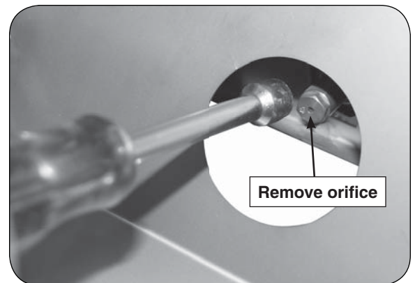
Fig. 24-3 Remove orifice to convert/check
