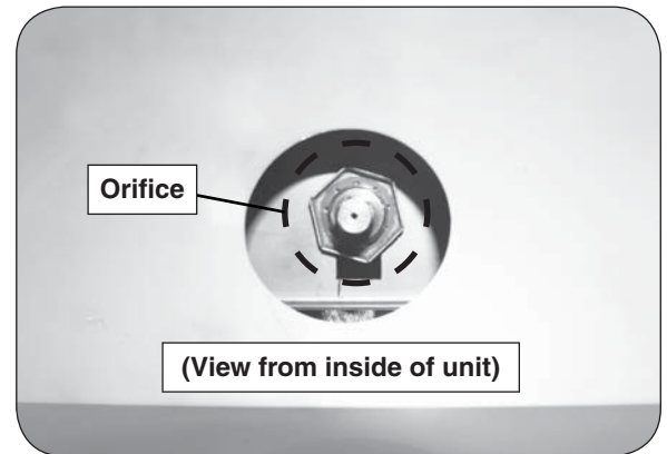
Fig. 24-2 Orifice location
