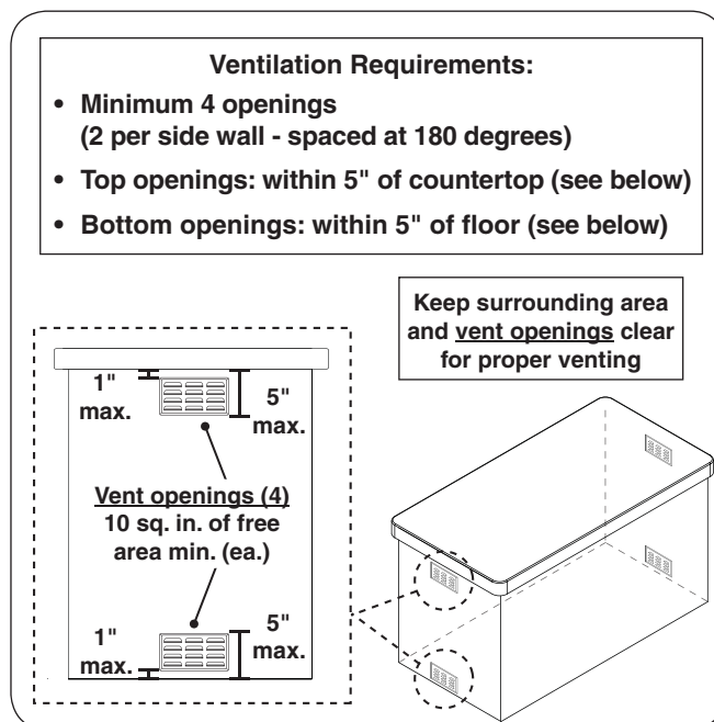
Fig. 11-1 Ventilation detail
