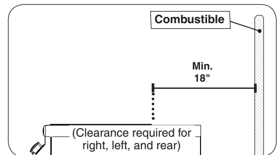
Fig. 9-4 Clearance 'C' Diagram
