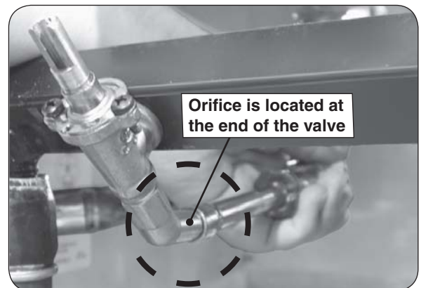
Fig. 21-3 Orifice location
