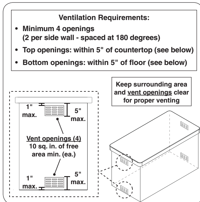
Fig. 11-1 Ventilation detail
