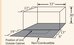
Recommended Framing Dimensions Zero Clearance Units
