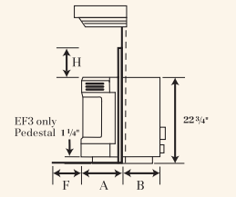
Side View - Insert
