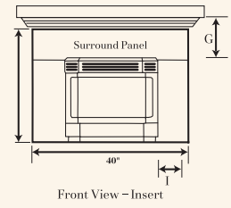
Front View - Insert
