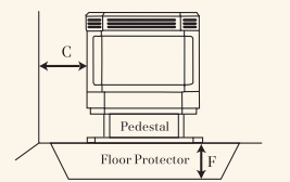
Front View - Free-Standing
